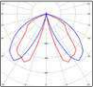
Models 2 to 4 LED 12W SYM Real light output - 797 lm CRI > 80
