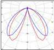
Models 1 and 5 LED 12W SYM Real light output - 680 lm CRI > 80
