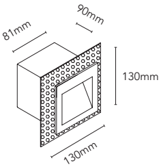
DELI 1 mounting box (Included)
