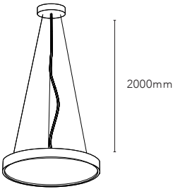
SUSPENSION KIT 2M
