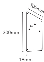
RØRHAT WALL MOUNT
