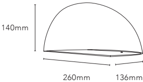
RØRHAT WALL LED
