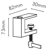
DARK CLAMP FOR T1/T2
