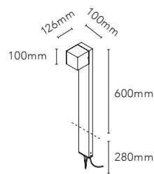
CUBE LED STAND
