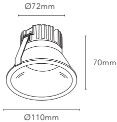
CURVE II Ø110
