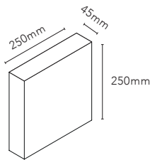
COMPACT DOWN W3
