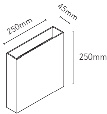
COMPACT UP/DOWN W3
